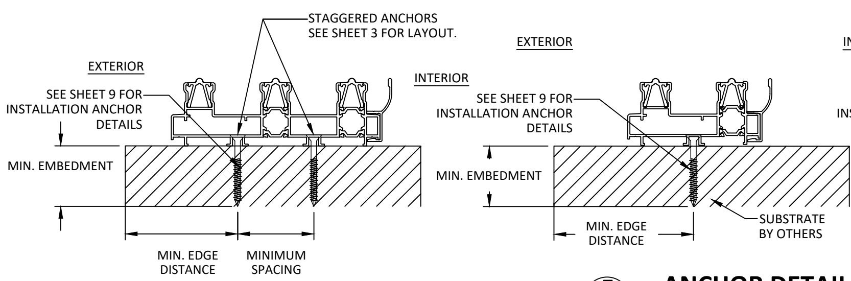
E 8 ANCHOR DETAIL THROUGH FRAME INSTALLATION (SILL) 3 TRACKS
