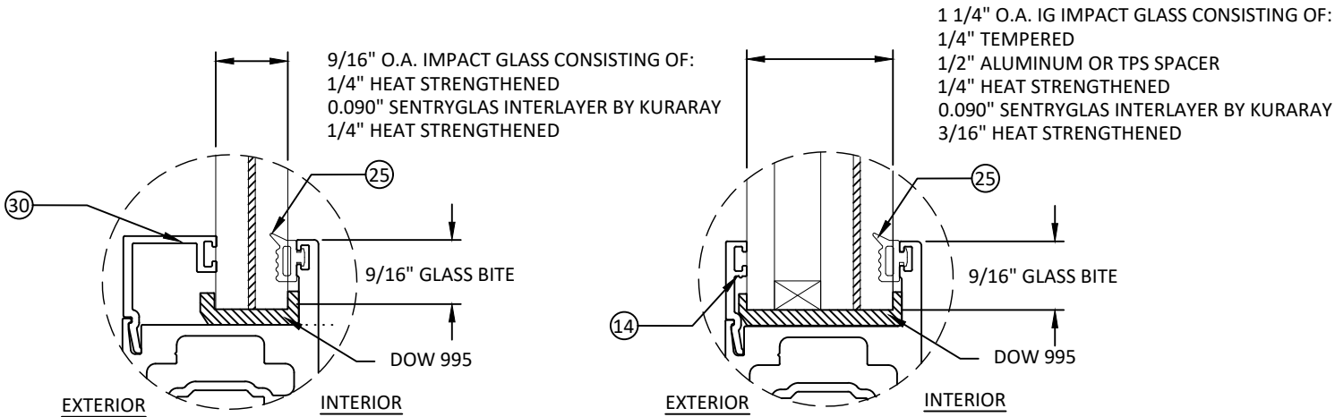
GLAZING DETAIL 1
