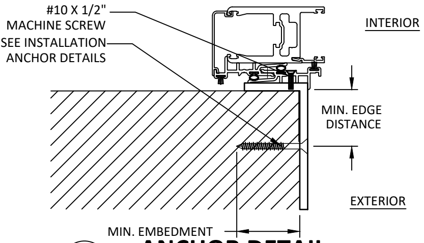
C 9 ANCHOR DETAIL INSIDE POCKET BRACKET INSTALLATION
